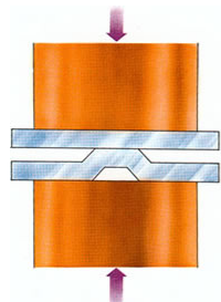
Projection resistance welding
